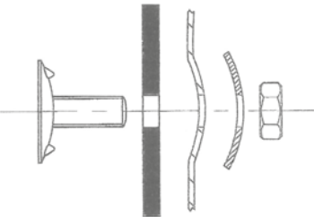
Elevator bucket installation with recessed elevator bucket bolt holes
