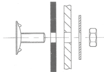
Elevator bucket installation with flat elevator bucket bolt holes
