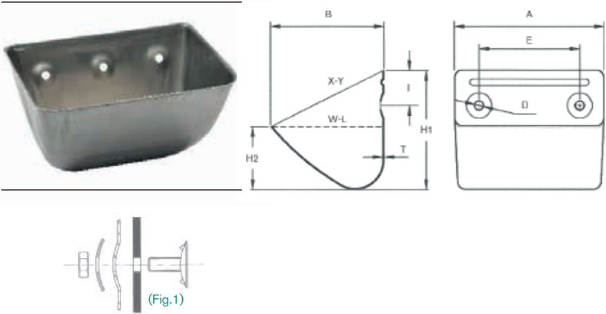
TECHNICAL SPECIFICATION - COLUMBUS STEEL ELEVATOR BUCKET
