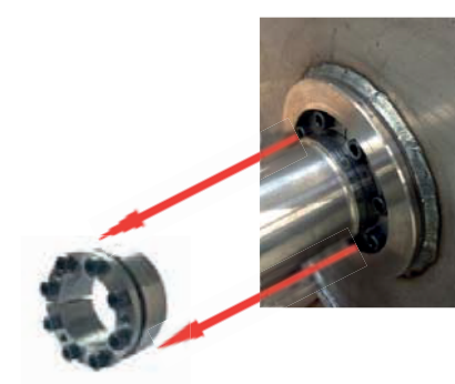
Shaft to drive pulley attachment by taper locking device
