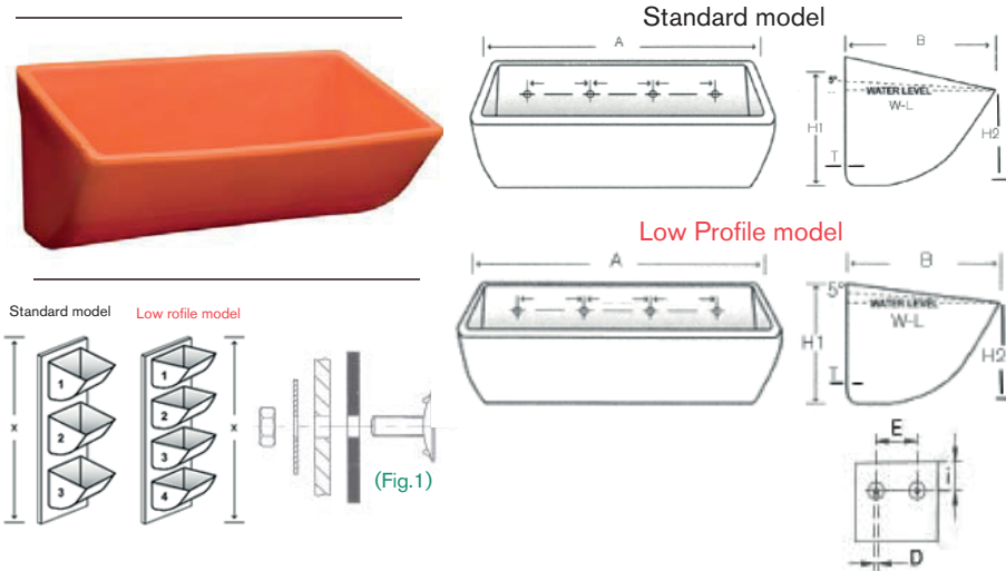
TECHNICAL SPECIFICATION - TIGER-TUFF® PLASTIC ELEVATOR BUCKET
