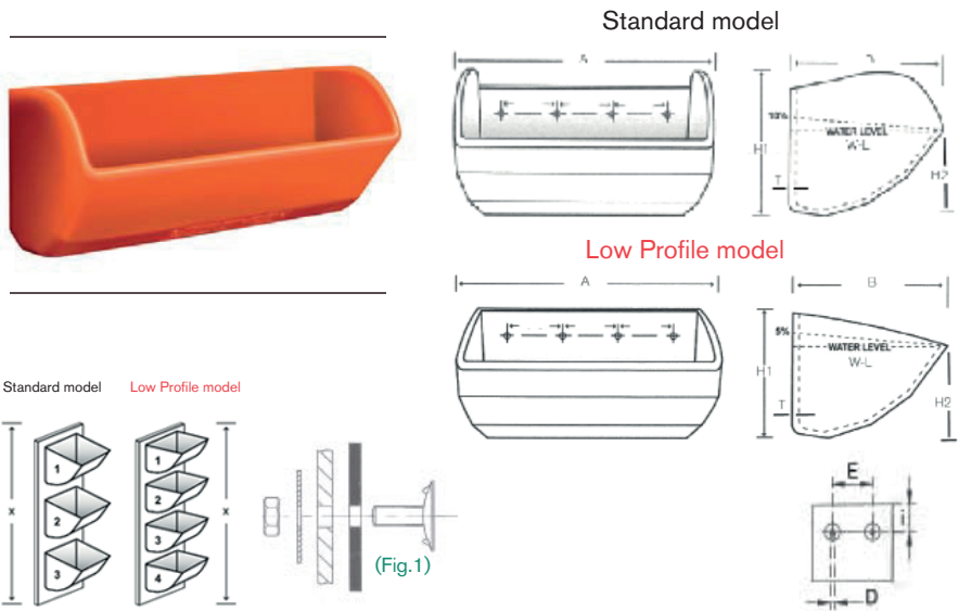
TECHNICAL SPECIFICATION - TIGER-CC® PLASTIC ELEVATOR BUCKET
