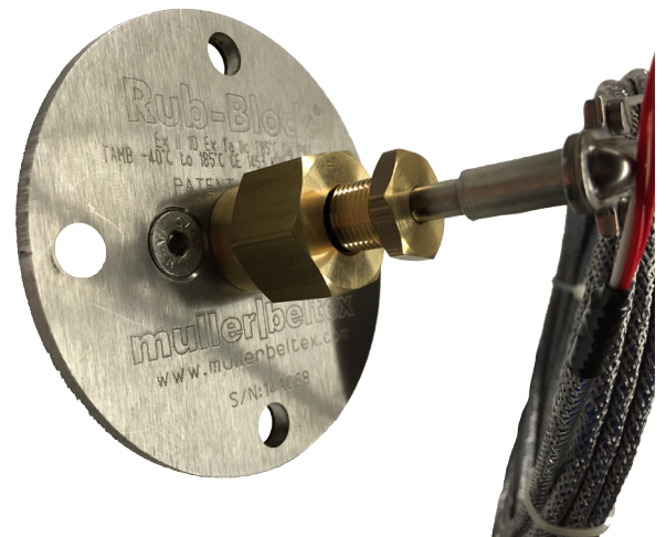
Step 2: Monteer de PT100 sensor in de messing behuizing
